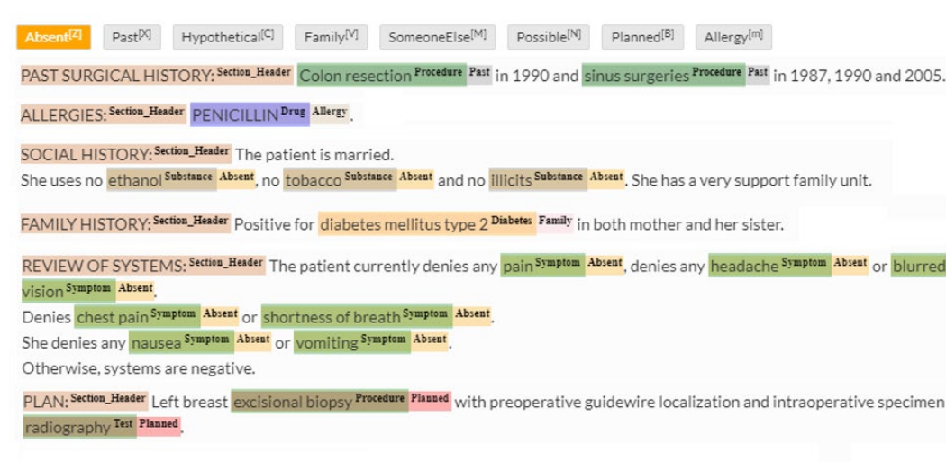
Figure 4. Annotation with examples of entity recognition and assertion labels
