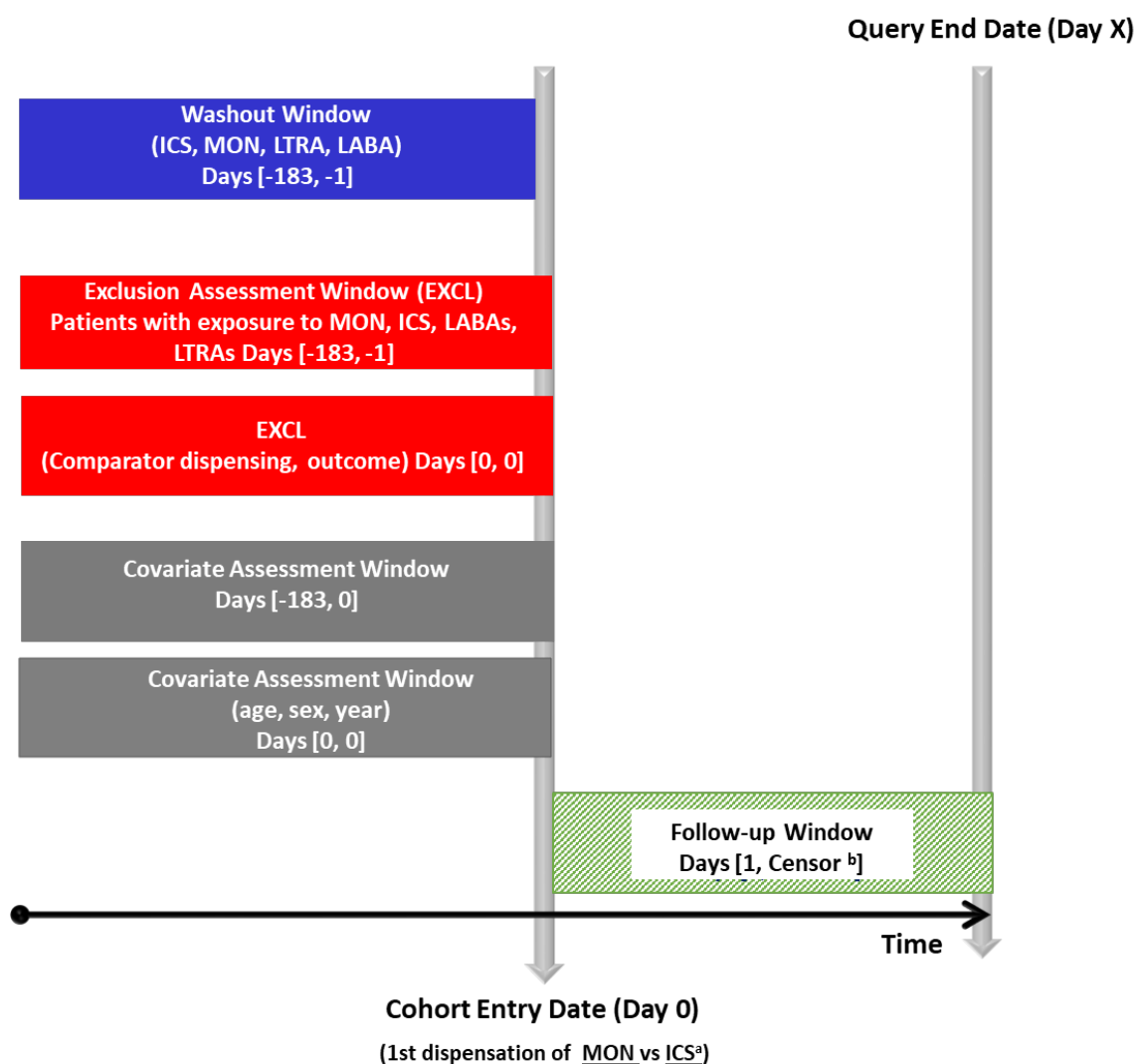
Figure 9. Study Design
