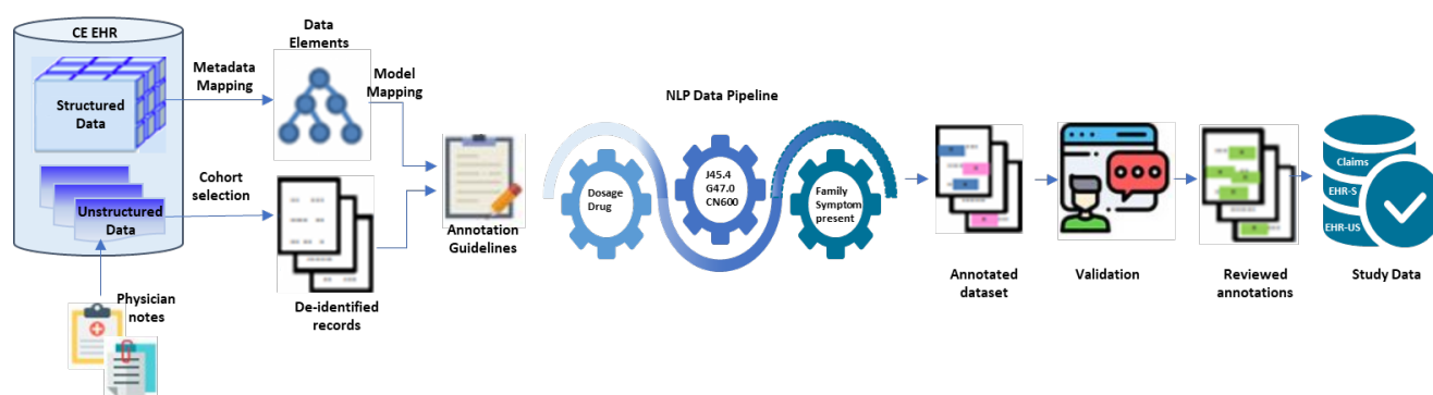
Figure 2. NLP Process
